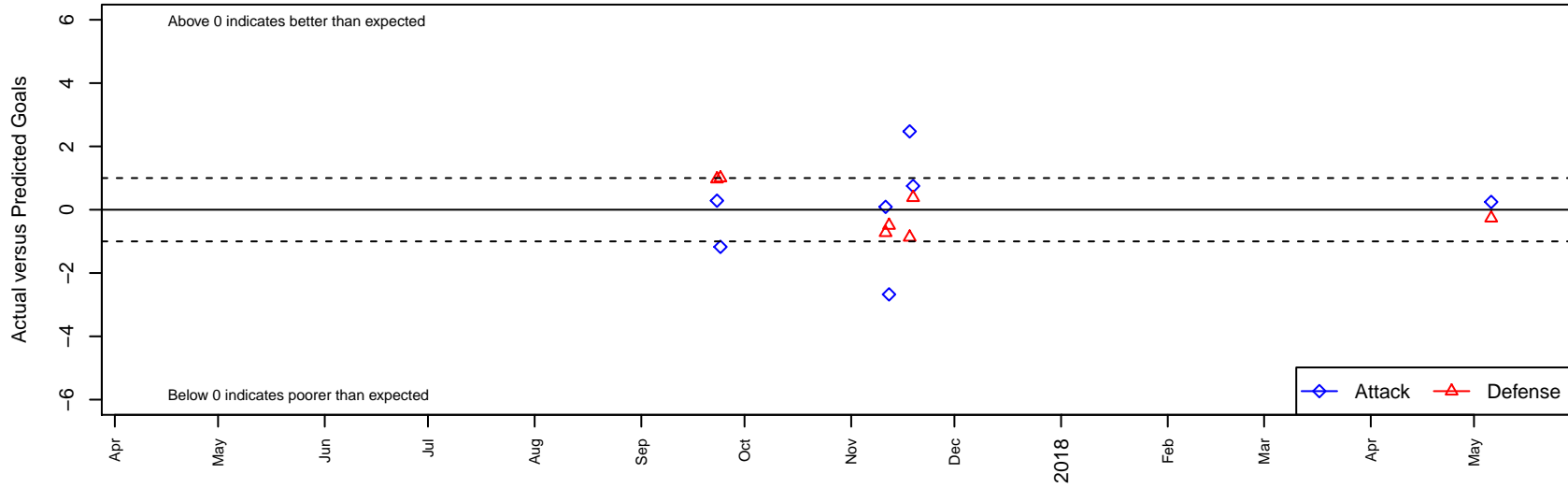
LA Galaxy USSDA B03 Dots are actual minus expected GF (blue circles) and GA (red triangles). Blue line is smoothed change in attack strength. Red is smoothed change in defense strength.
